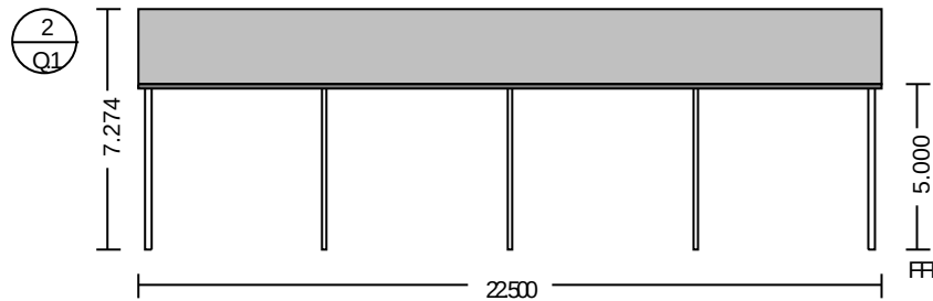
Left ELEVATION
