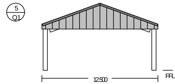
REAR ELEVATION
